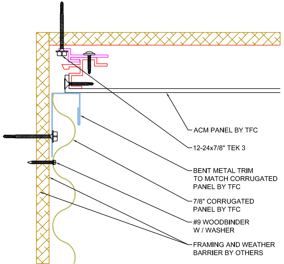
2 A4.0 DETAIL @ INSIDE CORNER (7/8" CORRUGATED) SCALE: 6" = 1' - 0"
