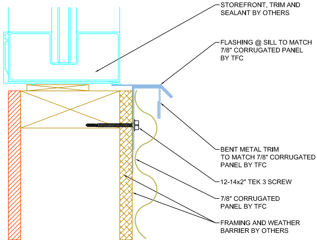
2 A4.0 DETAIL @ WINDOW SILL SCALE: 6" = 1' - 0"
