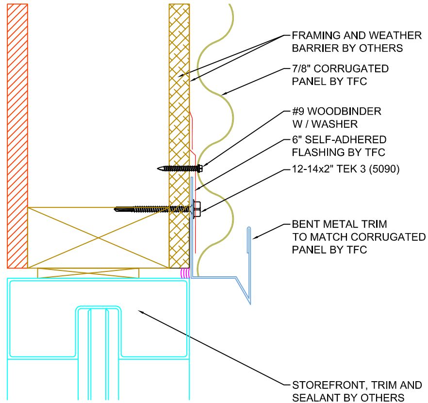
2 DETAIL @ WINDOW HEAD (7/8" CORRUGATED) A4.0 SCALE: 6" = 1' - 0"
