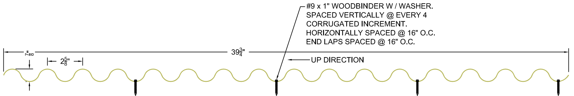
1 7/8" CORRUGATED PANEL PROFILE A4.0 SCALE: 3"=1'
