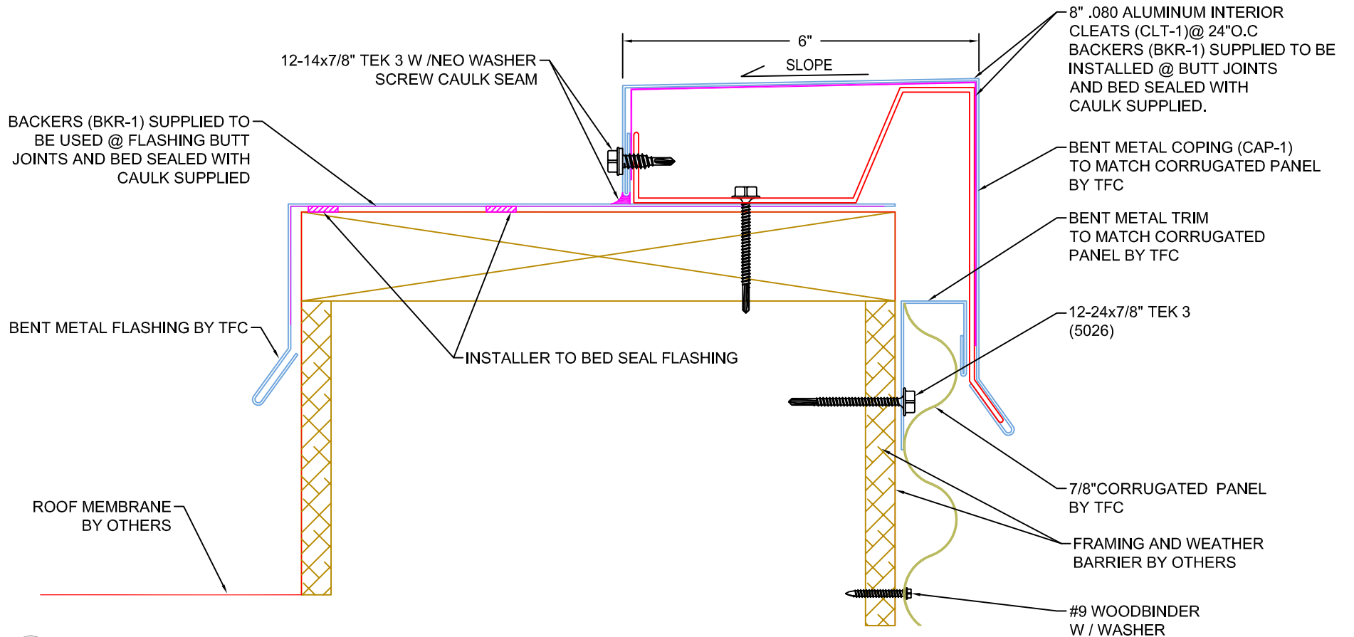
2 DETAIL 7/8" CORRUGATED @ BENT METAL COPING A4.0 SCALE: 6" = 1' - 0"
