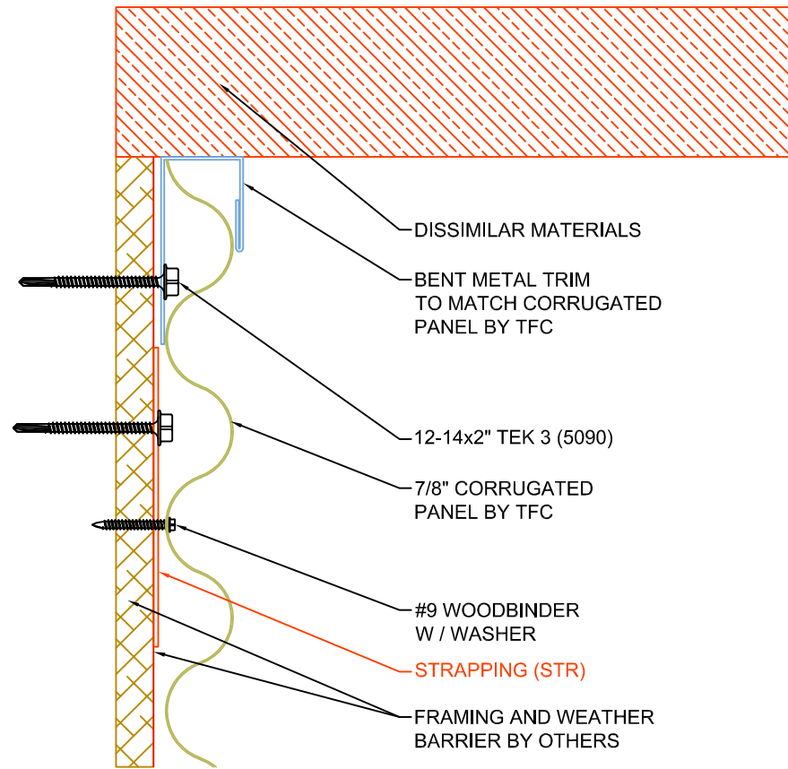
2 DETAIL @ DISSIMILAR MATERIALS (7/8" CORRUGATED) A4.0 SCALE: 6" = 1' - 0"
