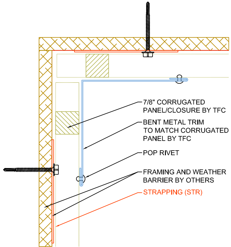
2 A4.0 DETAIL @ INSIDE CORNER (7/8" CORRUGATED) SCALE: 6" = 1' - 0"
