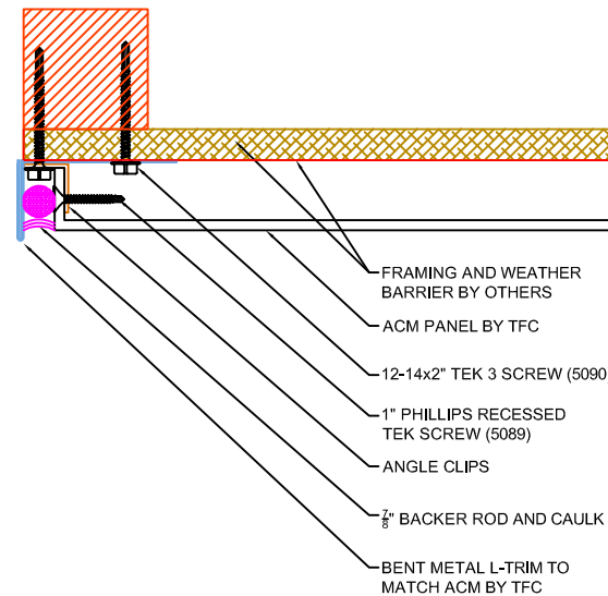
2 A4.0 DETAIL @ WET JOINT / END SCALE: 6\"/>
