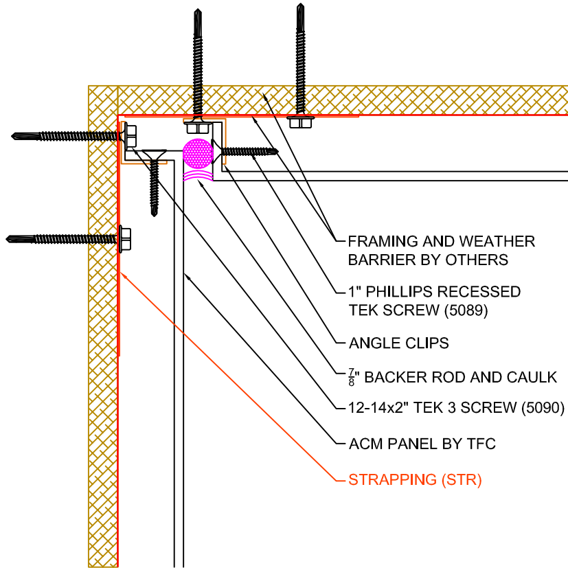
2 A4.0 DETAIL @ WET JOINT / INSIDE CORNER SCALE: 6" = 1' - 0"
