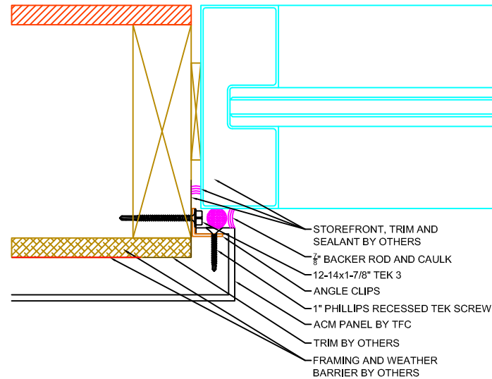
2 A4.0 DETAIL @ WET JOINT / WINDOW JAMB SCALE: 6" = 1' - 0"
