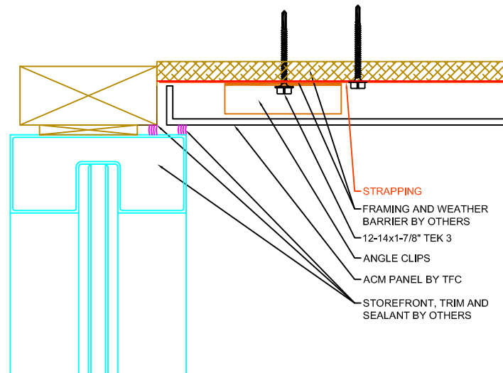
2 DETAIL @ WET JOINT / WINDOW HEAD A4.0 SCALE: 6" = 1' - 0"
