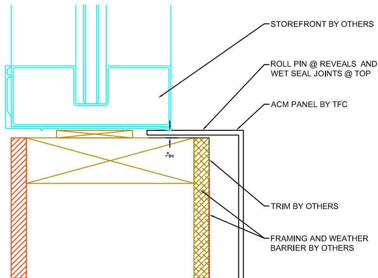
2 DETAIL @ WET JOINT / WINDOW SILL A4.0 SCALE: 6" = 1' - 0"
