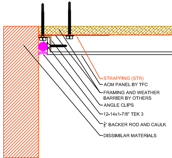
2 A4.0 DETAIL @ WET JOINT / END / DISSIMILAR MATERIALS SCALE: 6\"/>
