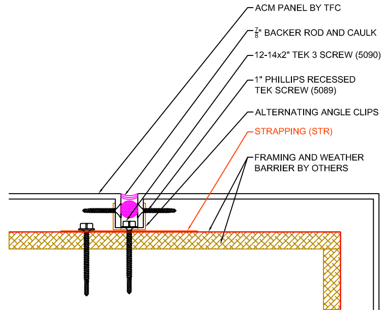
2 DETAIL @ WET JOINT / OUTSIDE CORNER FOLD A4.0 SCALE: 6" = 1' - 0"
