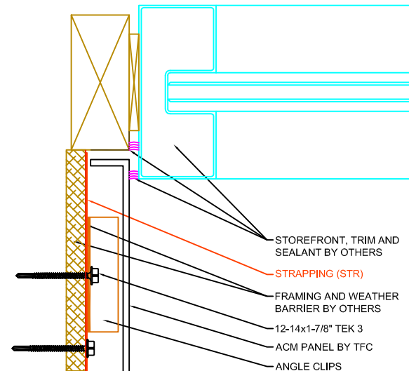
2 A4.0 DETAIL @ WET JOINT / WINDOW JAMB SCALE: 6" = 1' - 0"
