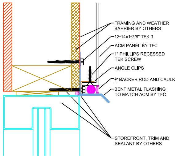
2 DETAIL @ WET JOINT / WINDOW HEAD A4.0 SCALE: 6" = 1' - 0"
