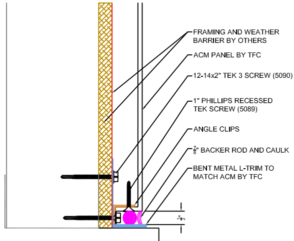
2 A4.0 DETAIL @ WET JOINT / BASE SCALE: 6" = 1' - 0"
