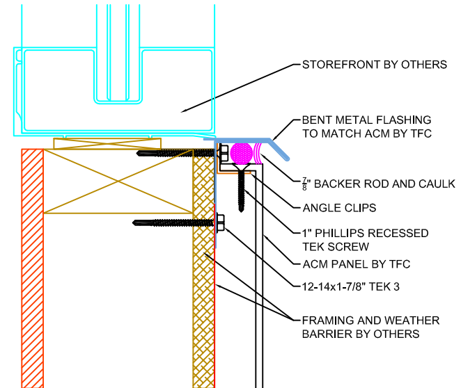
2 DETAIL @ WET JOINT / WINDOW SILL A4.0 SCALE: 6" = 1' - 0"
