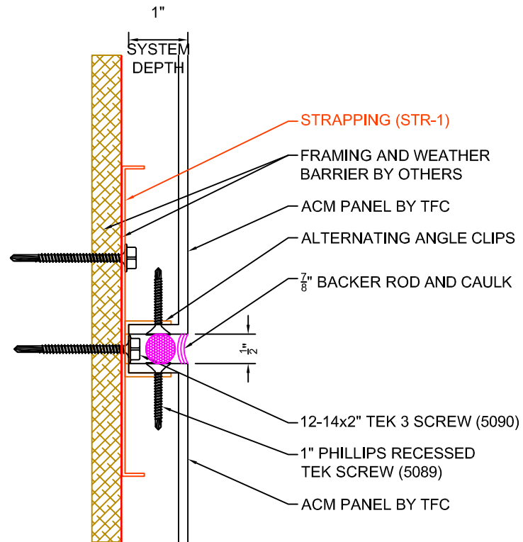
1 TYPICAL DETAIL @ WET JOINT/VERT. AND HORIZONTAL A4.0 SCALE: 6" = 1' - 0"
