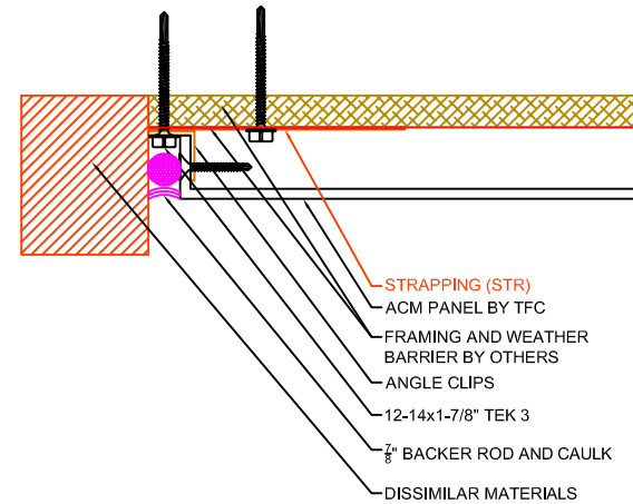
2 A4.0 DETAIL @ WET JOINT / END / DISSIMILAR MATERIALS SCALE: 6\"/>
