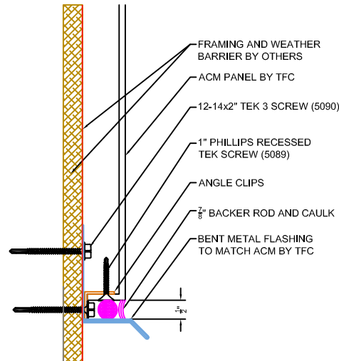
2 A4.0 DETAIL @ WET JOINT / FLASHING SCALE: 6" = 1' - 0"
