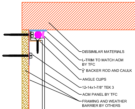
2 A4.0 DETAIL @ WET JOINT / END / DISSIMILAR MATERIALS SCALE: 6\"/>
