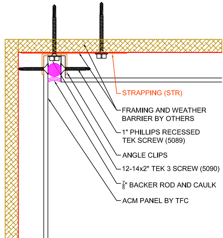
2 A4.0 DETAIL @ WET JOINT / INSIDE CORNER SCALE: 6" = 1' - 0"
