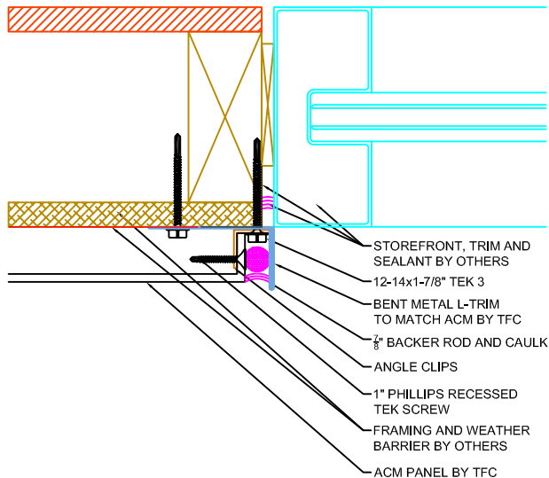
2 A4.0 DETAIL @ WET JOINT / WINDOW JAMB SCALE: 6" = 1' - 0"
