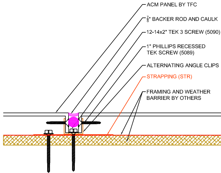
2 DETAIL @ WET JOINT / TOP A4.0 SCALE: 6" = 1' - 0"
