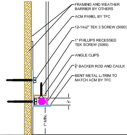
2 A4.0 DETAIL @ WET JOINT / BASE WITH KICKPLATE SCALE: 6" = 1' - 0"
