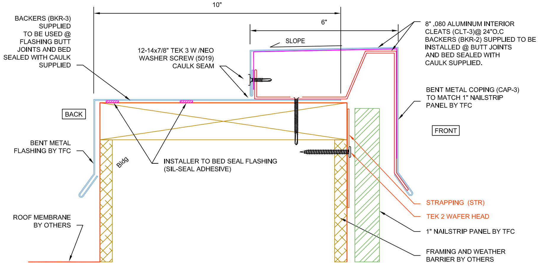
2 DETAIL @ BENT METAL COPING A4.0 SCALE: 6"=1'-0"
