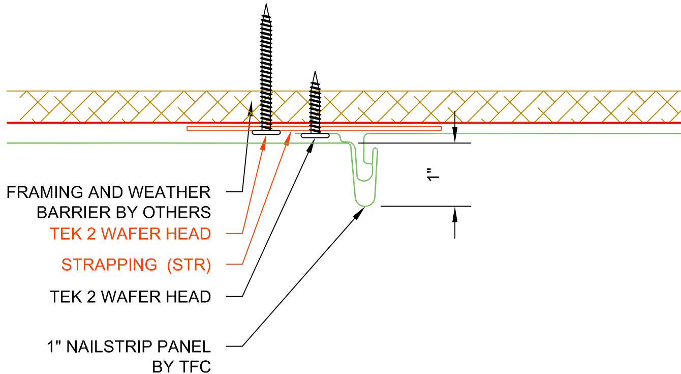
1 TYPICAL PLAN DETAIL @ 1" NAILSTRIP PANEL A4.0 SCALE: 6"=1'-0"
